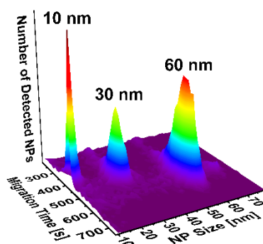
Figure 1: CE-ICP-MS electropherogram of a mixture of NIST AuNP reference materials.
